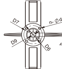
HB950/S-EH/ RH 14" – 24"
